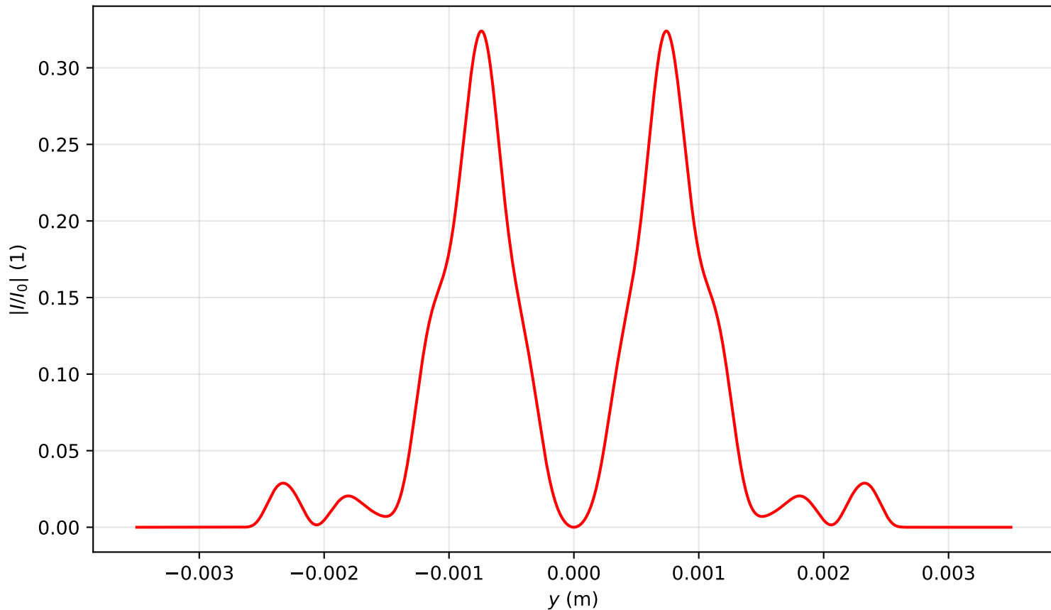
Intensity profile I(x=0, y, z=3.423)/I_0 , \text{Pin}=6.0\text{Pcr} , artificial time
